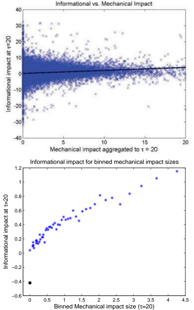
FIG. 9: The informational impact at \tau = 20 vs. mechanical impact integrated up to \tau = 20 , S_{20}^M(t) . In (a) the dots correspond to individual transactions, and the line is a regression using ordinary least squares. In (b) the data is binned based on the integrated mechanical impacts, illustrating that even though the relationship is noisy, the correlation increases consistently with increasing size. Note that the black square corresponds to the case where the mechanical impact is strictly zero.
