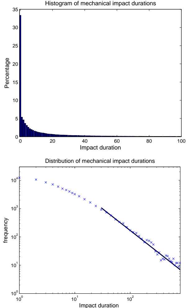
FIG. 5: Distribution of mechanical impact durations. The top panel is the probability of each duration, and the bottom panel covers a longer time period on double logarithmic scale. The x's correspond to the empirical measurements, and the line to a fit using ordinary least squares.
