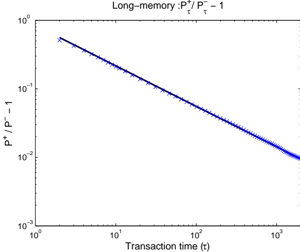
FIG. 7: An illustration of the long-memory of order signs. The ratio P_{\tau}^{+}/P_{\tau}^{-} - 1 is plotted on double logarithmic scale (x's) and compared to a power law (line) with exponent \gamma = 0.59 .
