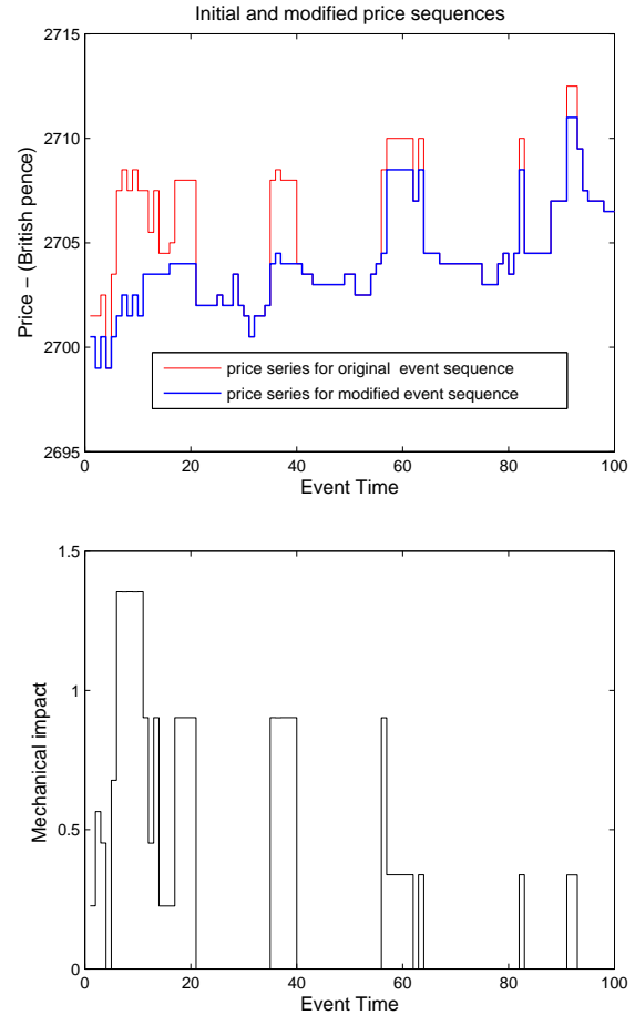
FIG. 1: (a) Initial and modified price sequences for the removal of a buy market order and (b) the resulting mechanical impact (which is just the difference between the two price series in (a)). Note that this figure and all other figures in this paper are based on the stock AZN. Prices are in pence and impacts are in units of average spread.
