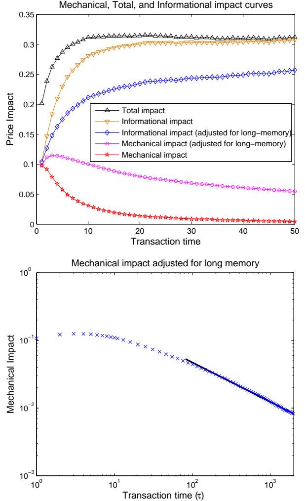
FIG. 8: (a) A comparison of the average mechanical, informational, and total impacts with and without adjustments for long-memory. In ascending order we show the average mechanical impact R^M(\tau) , the mechanical impact C(\tau) adjusted for long-memory, the informational impact adjusted for long-memory R^T(\tau) - C(\tau) , the informational impact R^T(\tau) - R^M(\tau) , and the total impact R^T(\tau) , all as a function of time. In (b) we show C(\tau) over a longer time period in double logarithmic scale.
